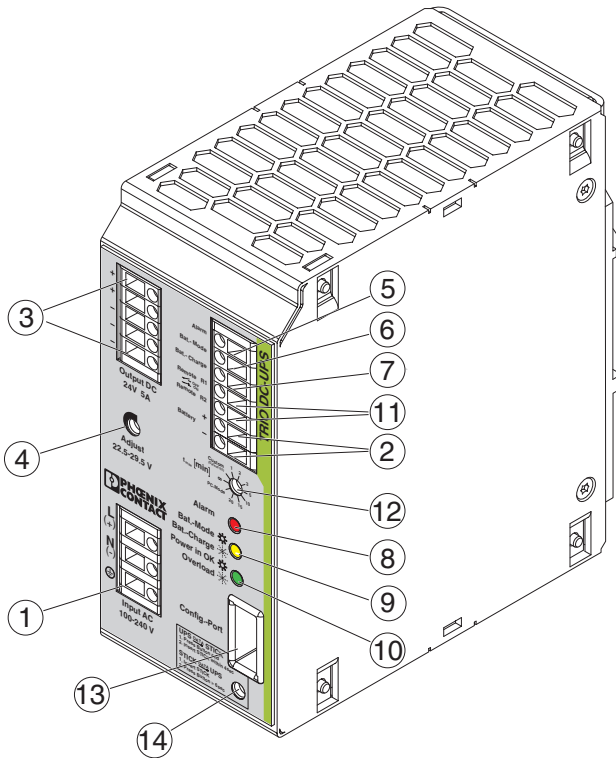
Figure 1 TRIO-UPS/1AC/24DC/5 structure
